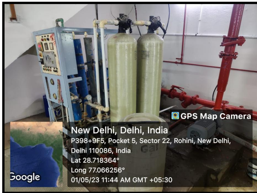
Water Treatment Plant in the Campus
