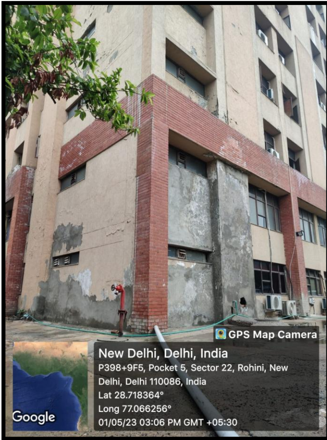
Pipe from the Roof attached to the Tank collecting Rain Water
